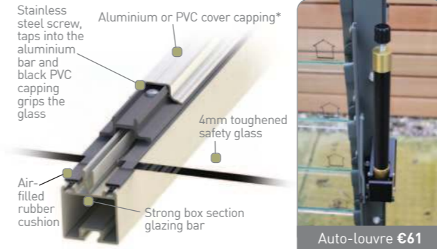
Auto-louvre €61
